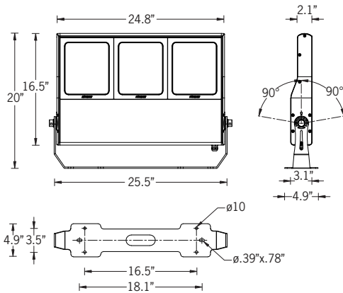
Mounting Detail
